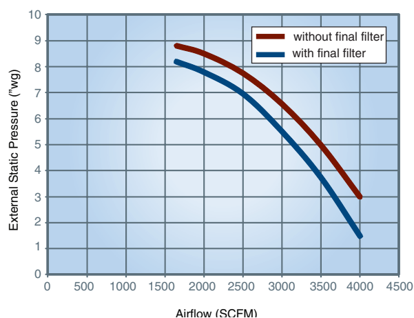
WSO 25-2 (7.5 HP)
