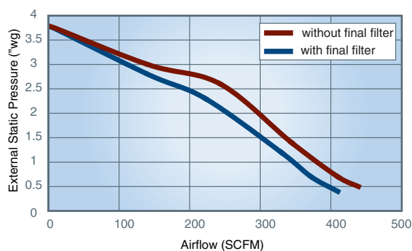
WSO 10* (3/4 HP)
