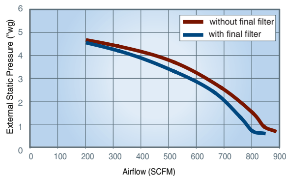
WSO 15* (1-1/2 HP)
