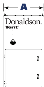
Front View
